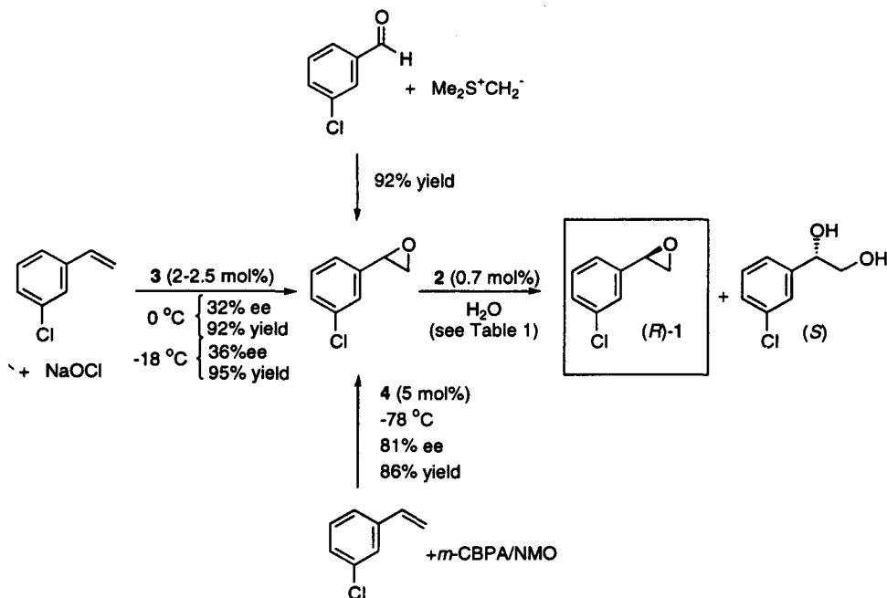
Scheme 1. Synthesis of enantiopure 1 .
